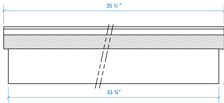
Detail B: Inner Tray Support (make 8)
